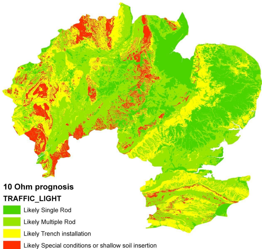
Figure 4 - Typical effect of soil/geology variations on earthing installations
