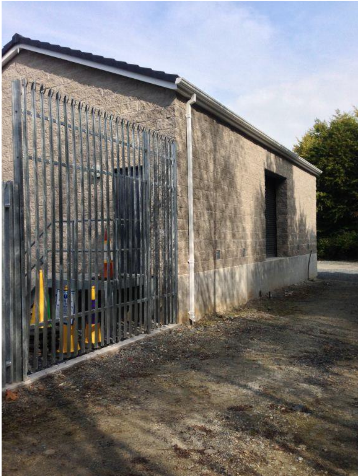
High voltage switch room under construction on a raised plinth. (Courtesy NIE)
