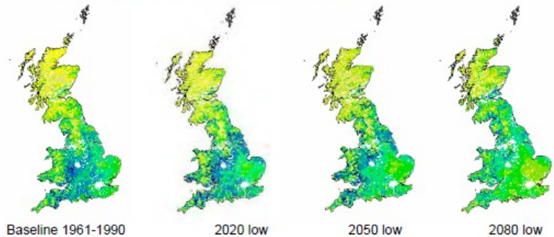
Figure 3.1 The suitability of different areas of the UK for beech under low and high emissions scenarios for 2020, 2050 and 2080
