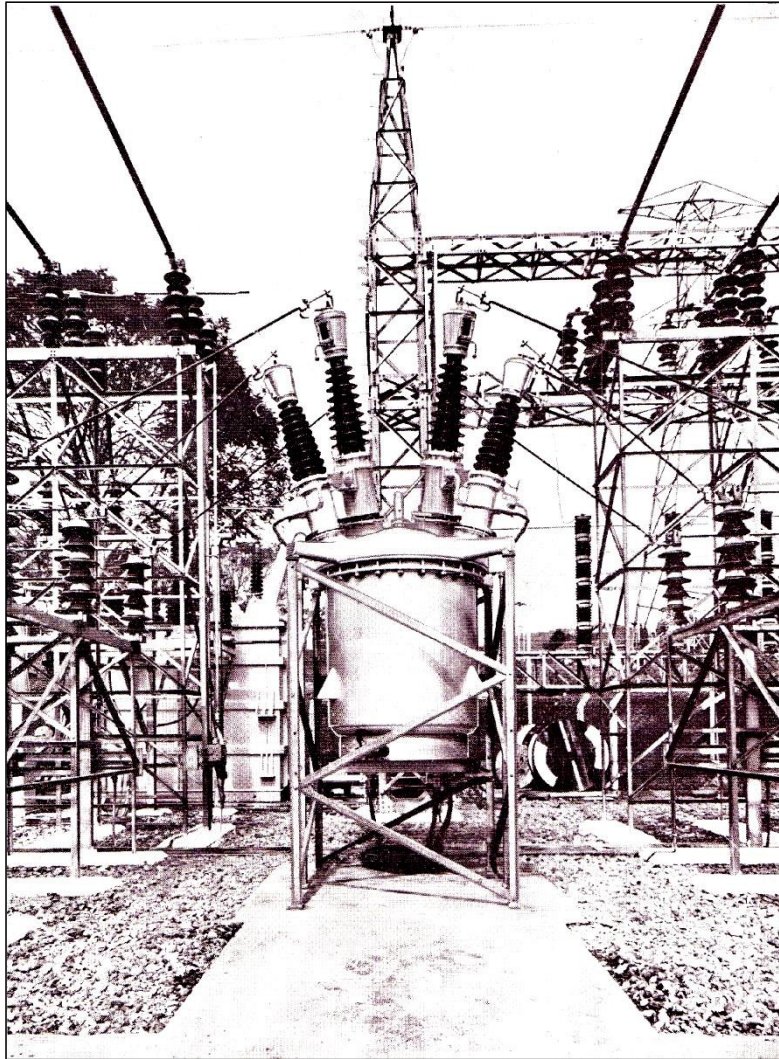
Photograph 9 - Rated at 750MVA this Type JB429 oil circuit-breaker is in service on the 66kV system of the Central Electricity Board, Malaya
