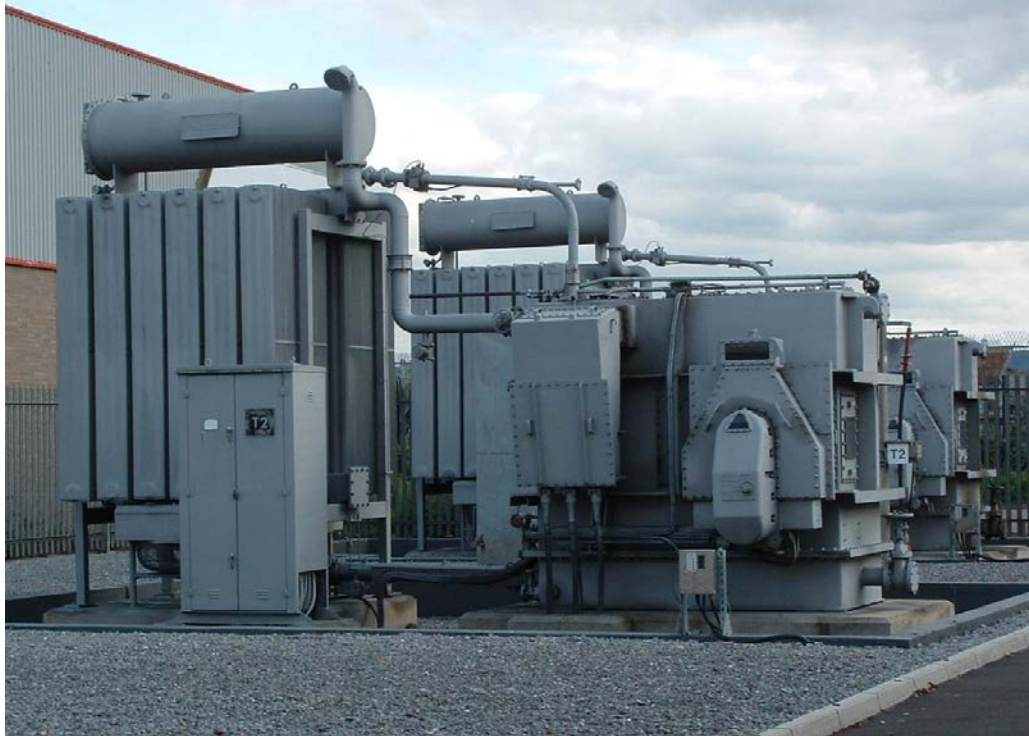
Examples of 33k / 11kV ground mounted (GM) transformers (two visible in photo) with coolers shown to the left of the picture.
