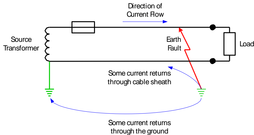
Figure 3 - Earth fault current path
